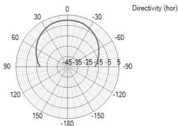
Hor. 4005 Hz, DI=10.0 dB
