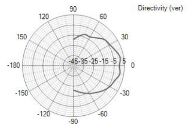
Ver. 4005 Hz, DI=10.0 dB
