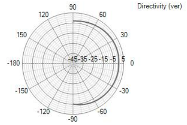
Ver. 250 Hz, DI=4.5 dB
