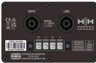
INPUT PANEL
